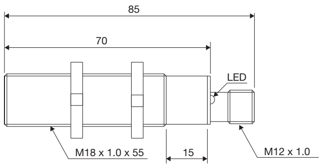
Fig. 8 Conector CA18CAF...M1IO
